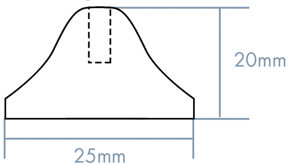
Plunger Pad
